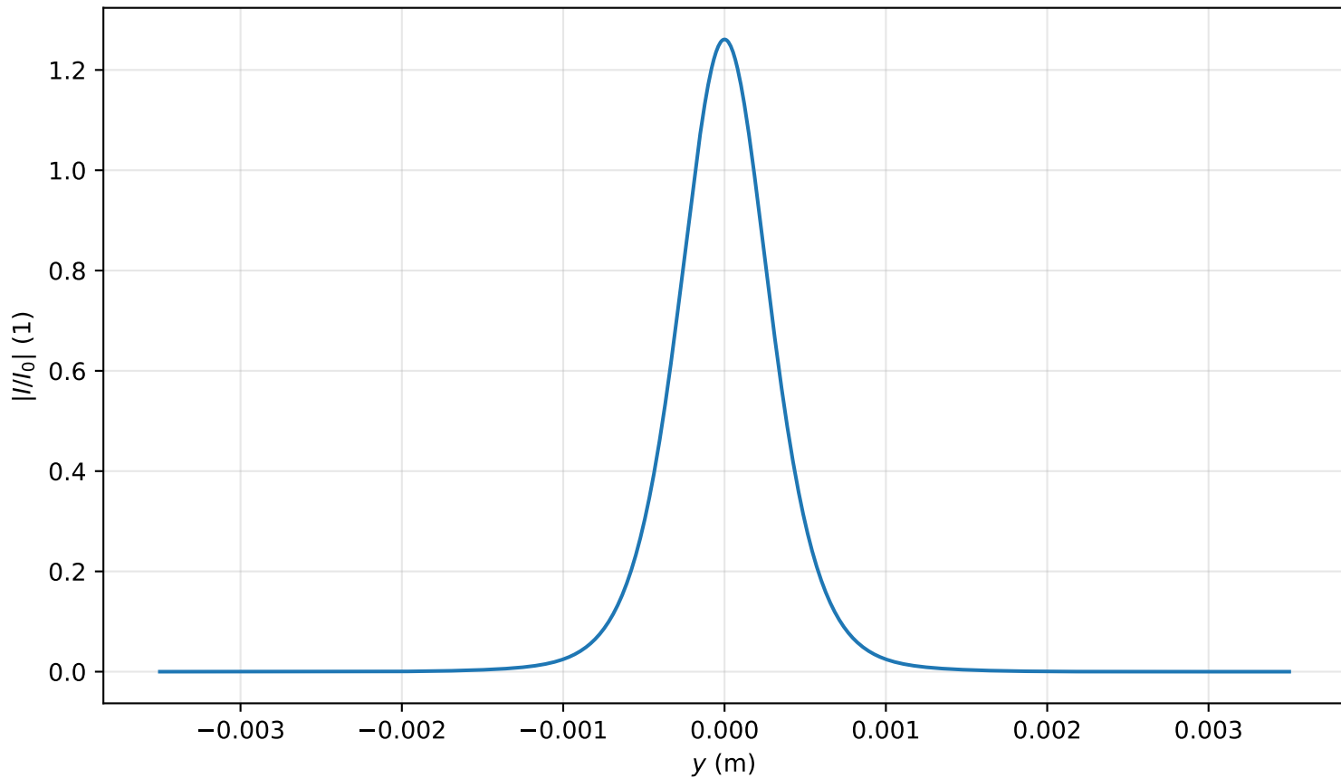
Intensity profile I(x=0, y, z=2.309)/I_0 , P_{in}=0.8P_{cr} , artificial time
